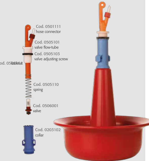
Jumbo 98 drinker is supplied with 3 m hose and shut-off saddle
